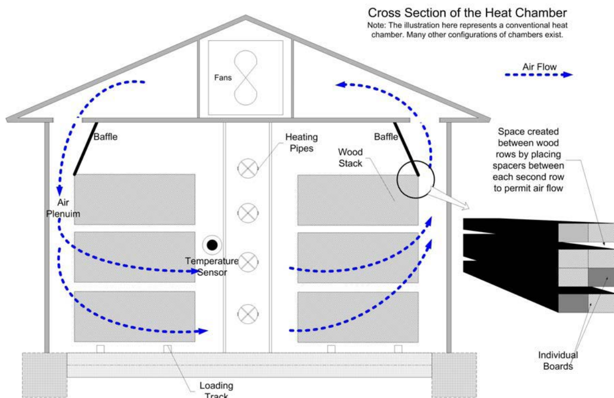
Figure 2: A type of heat chamber with the heating pipes in the middle. Temperature sensors should be placed at a location where the air exits the wood stack and is therefore likely to be the coolest.
