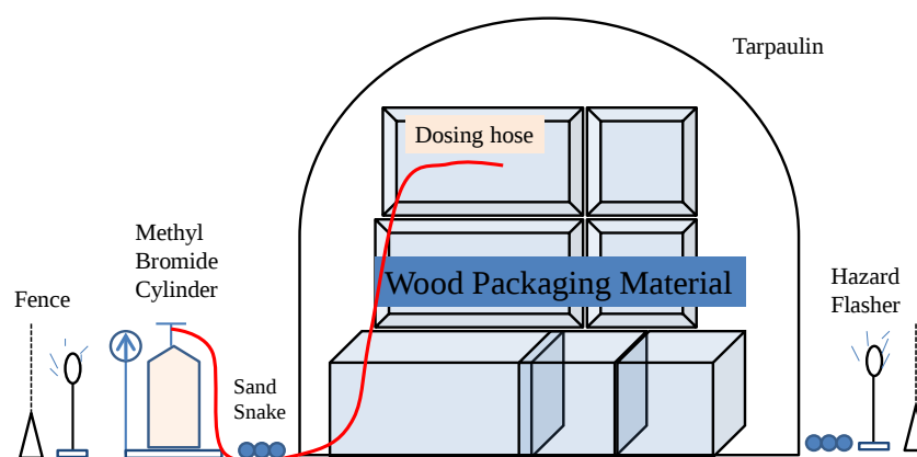
Figure 6: Common Layout of Tarpaulin Fumigation
