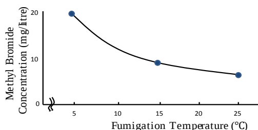
Figure 3 Effects of temperature on Methyl Bromide dose required to achieve LC99 after 24hrs fumigation.
