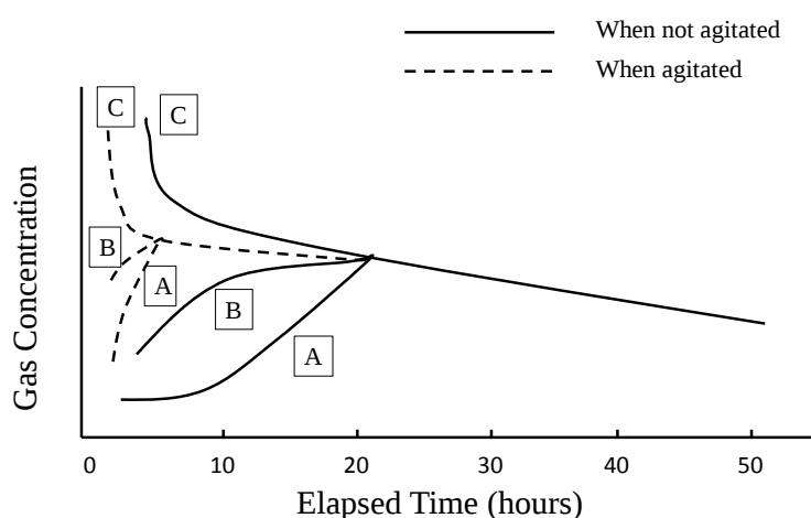
Figure 4 Gas diffusion in a fumigation chamber over time: A-Upper, B-Middle, and C-Lower chamber gas probes
