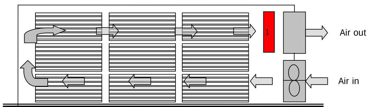
Figure 5: A heating chamber in which heating occurs at the floor of one-side. The temperature sensor is placed at the air exits the wood stack (marked “1”).
