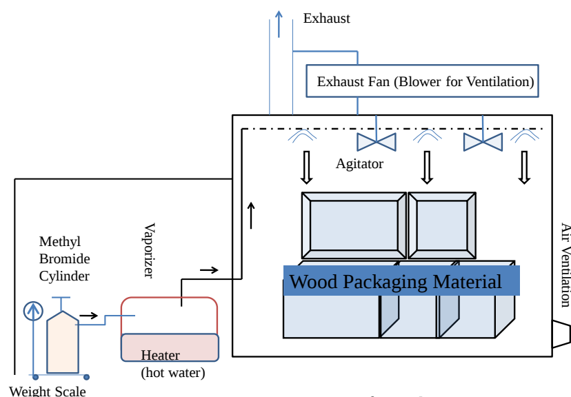
Figure 5: Common Layout of Warehouse Fumigation
