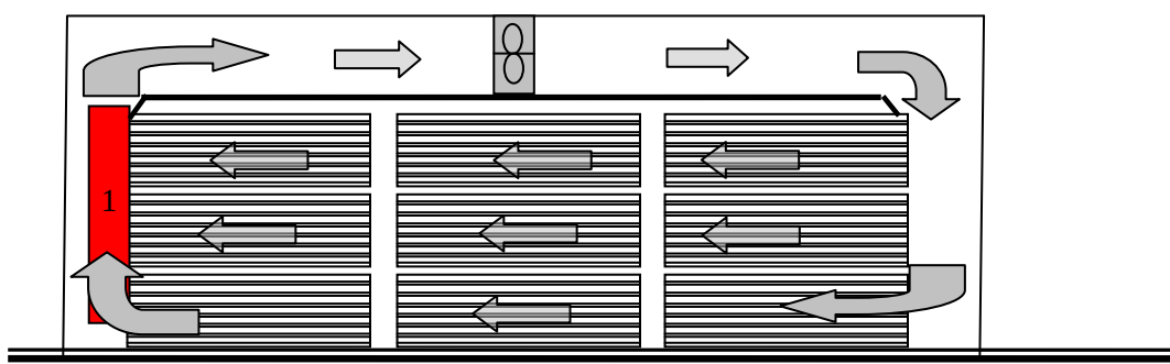
Figure 3: A heating chamber in which the heating pipes are located with a fan above the wood stack. The cold spot is likely to be nearest the exit side of the stack and the temperature sensor should be placed where the air exits the wood stack (marked "1").
