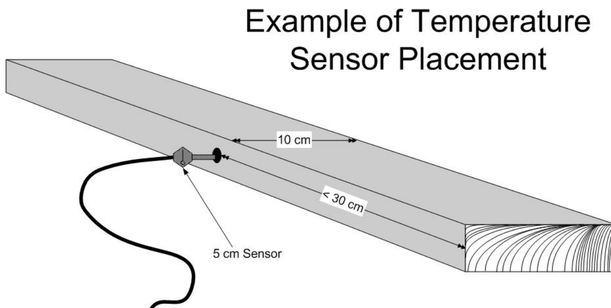
Figure 6: An example of a temperature sensor placement in a wood plank.
