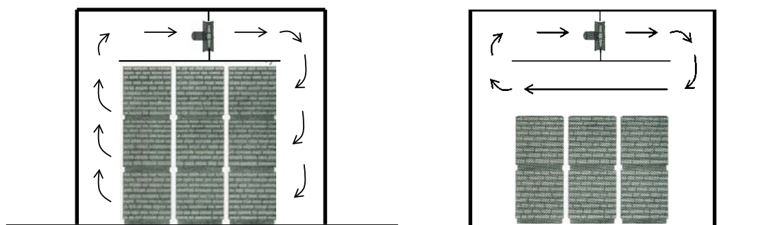
Figure 1: Schematic illustration of a loaded heat chamber resulting in different air circulation. Left: with a completely stockpiled chamber (cross section), the air circulates through the entire stack and heating is more uniform. Right: in an incompletely stockpiled chamber (cross section), the air circulates over the wood stack and the wood is not heated as quickly as the free space in the chamber.
