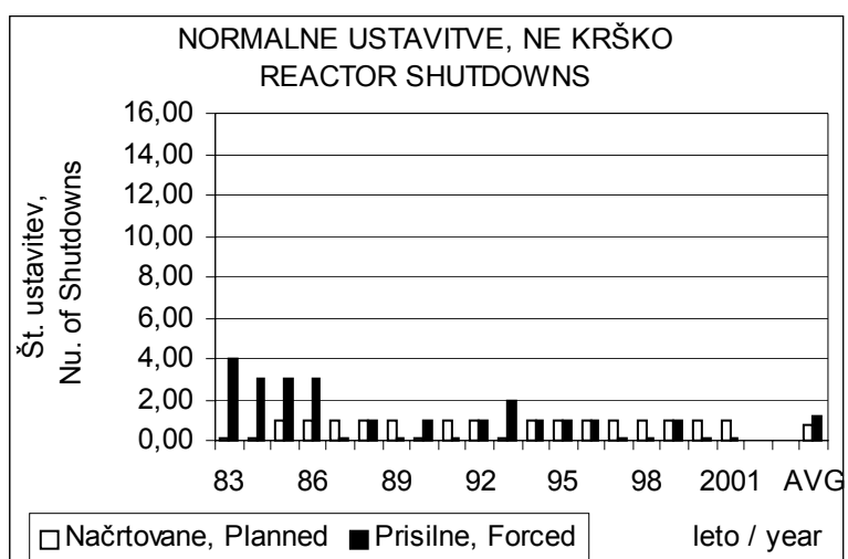
Figure 2.5: Reactor shutdowns.
