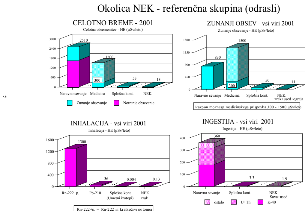
Figure 3.7: Dose assessment for adult residents of the reference group in the vicinity of NPP Krško in the year 2001.
