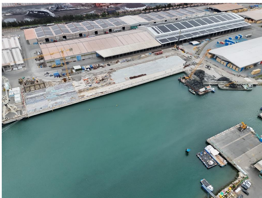
Building new berth No. 12 – Basin 2 (source: Port of Koper)
